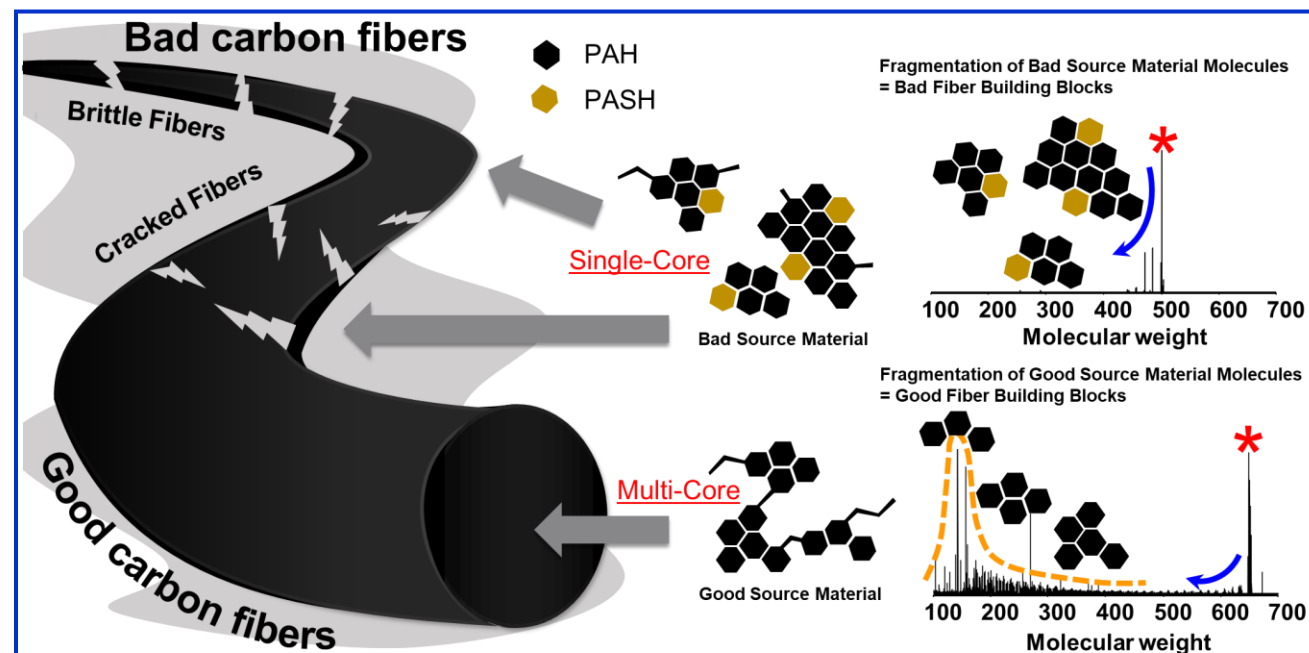
Figure 1. Gas-phase fragmentation mass spectra (MS/MS) for bad (top right) and good (bottom right) source materials for carbon fiber production. Bad source material molecules contain abundant single-core molecules comprised of high-molecular-weight PAH and PASH, which produce no stable carbon fibers upon spinning. Conversely, good source material molecules contain abundant multicore compounds composed of low molecular weight, interconnected PAH and produce good carbon fibers. Bad source materials are identified in FT-ICR mass spectra by production of high mass fragments (upper right, blue arrow). Good source materials are identified by production of low mass fragments (bottom right, yellow dashed line).
