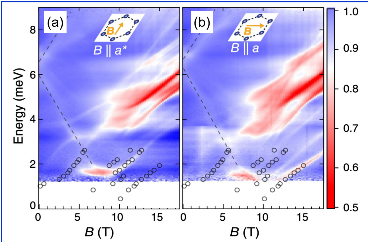
Figure: Normalized far-infrared transmission (see color legend) measured on a single-crystal of \text{Na}_2\text{Co}_2\text{TeO}_6 at T = 5\text{K} , with the applied magnetic field \mathbf{B} \parallel \mathbf{a}^* (panel a) and \mathbf{B} \parallel \mathbf{a} (panel b). Black circles are excitation modes extracted from the EPR spectra measured on powdered samples at T = 5\text{K} . Dashed lines are guides to some of the weaker excitation modes.
