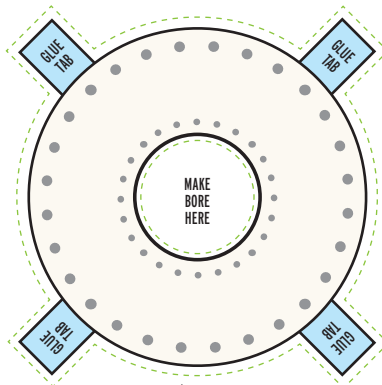
21.1 T MAGNET BOTTOM
