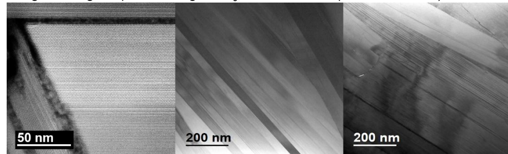
Figure 2: Transmission Electron Microscope (TEM) images of the three wires showing grains and grain boundaries. Our results showed that the wire with the lowest J_c of only 684 A/mm 2 (measured at 4.2K and 15T) had high a -axis alignment but also had amorphous content at its grain boundaries, which acted as a current transport barrier and thus significantly lowered the J_c of the wire.
