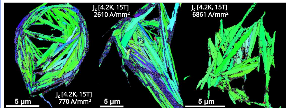
Figure 1: Electron micrograph of the cross sections of three Bi-2212 round wires with widely varying critical current densities ( J_c ) showing their a -axis grain alignments. The wire with the best a -axis alignment (far right, highest proportion of grains in green) had the highest J_c of 6861 A/mm 2 (at 4.2K and 15T).
