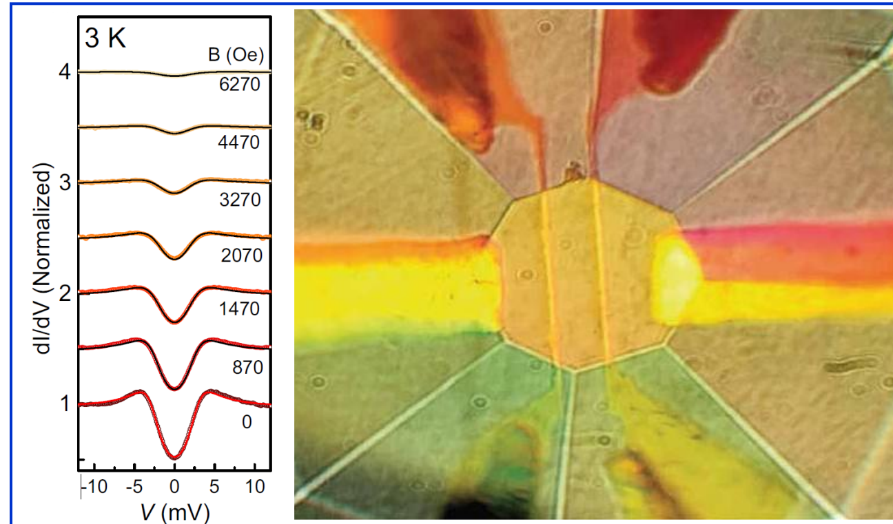
Figure 1. a , The change of differential conductance in response to applied voltage. The drop that forms near 0 mV is due to the opening of the superconducting gap. Vertical spectra are offset by increasing magnetic fields values shown on the right. b , An image of the tunneling circuit formed on the tip of the diamond anvil press.
