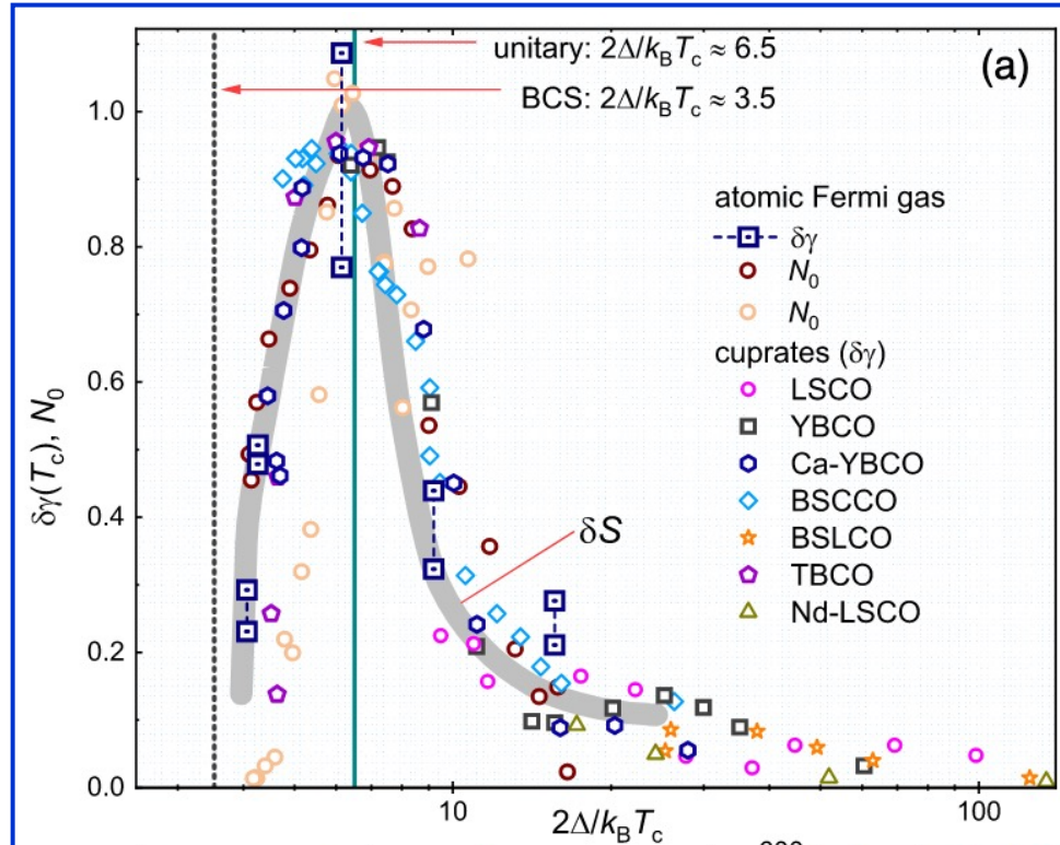
Figure: A comparison of the jump \delta\gamma at T_c in the specific heat coefficient for seven different cuprate superconductors, with the equivalent quantity in a cold atomic gas. Also shown are the change in entropy \delta S and the condensate fraction N_0 . All quantities are plotted versus the gap ratio, 2\Delta/k_B T_c . The common peak at 2\Delta/k_B T_c \approx 6.5 indicates a “magic gap ratio” at a crossover from BCS to BEC condensation.
