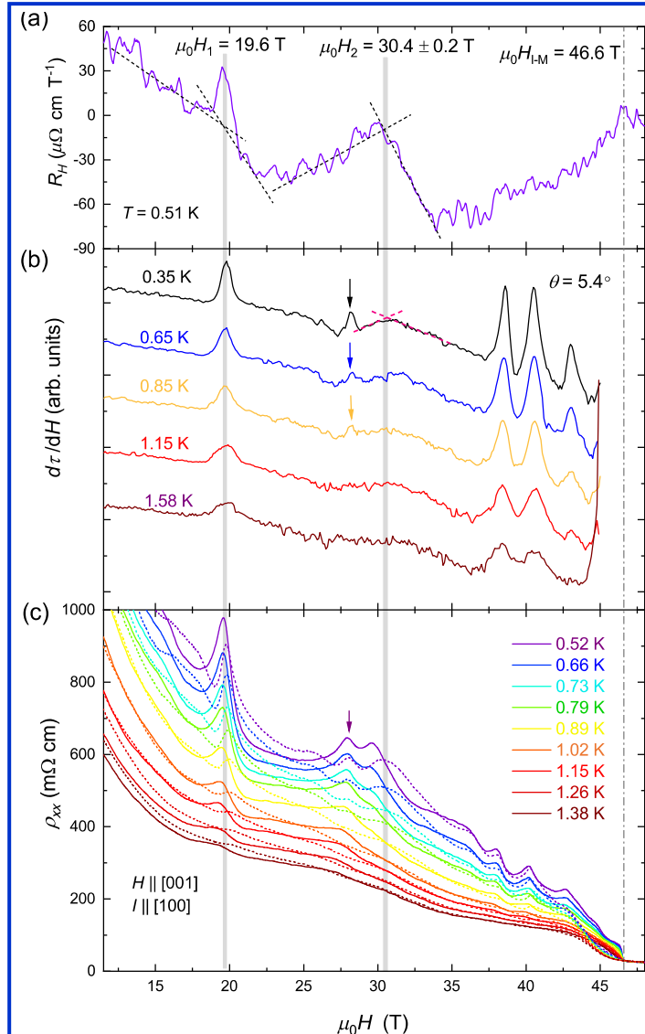
Figure: A comparison of (a) Hall effect, (b) magnetic torque, and (c) electrical resistivity in the Kondo insulator \text{YbB}_{12} confirms that quantum oscillations and phase transitions show up in all three physical measurements at the same magnetic fields.
