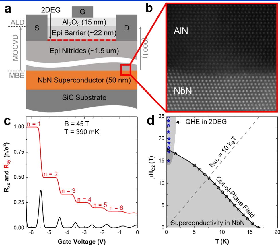
Fig.1 (a) Layer structure of the epitaxial nitride heterostructure. (b) High-resolution transmission electron microscopy image of the semiconductor /superconductor interface. (c) The quantum Hall effect in the GaN semiconductor. (d) The temperature and magnetic field region where superconductivity in NbN and the quantum Hall effect in GaN coexist.
