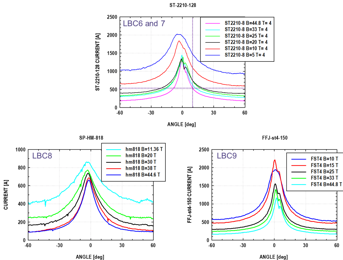
Fig. 4.1.12 Torque I_c measurement results of REBCO samples of recent LBC6—9 tapes via the NHMFL 45T 32mm (19mm room temperature bore) hybrid magnet, the world's first I_c(Q,B,T) measurement at 45T.
