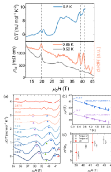
Figure 2.3.5 Quantum oscillations in the Kondo insulator YbB12. Top: Heat capacity C/T (blue) and electrical resistivity \rho_{xx} and derivative of the torque \tau vs B (red, grey) as a function of magnetic field at sub-kelvin temperatures, measured in the 41.5T resistive and 45T hybrid magnets. Dashed lines indicate quantum oscillation maxima visible in all three quantities. Bottom: (a) Oscillatory component of C/T at temperatures from 0.8K to 3K, revealing a distinctive double-peak structure. (b) Landau fan diagram confirming oscillation frequencies of 41.1T and 36T. (c) Effective mass determined from the temperature dependence of the oscillation amplitudes in heat capacity (red) and torque magnetometry (blue and purple), yielding consistent values of approximately 5-7 free electron masses. The observation of quantum oscillations in the heat capacity -- a bulk thermodynamic quantity -- provides direct evidence that neutral fermions in the bulk, rather than surface states, are responsible for the metallic-like quantum oscillatory behavior in this electrical insulator.
