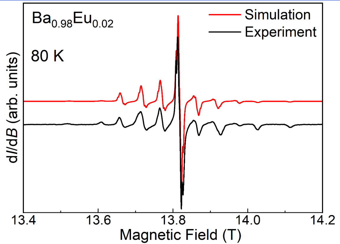
Figure 1. High-field EPR spectrum (Experiment) recorded at a frequency of 385GHz along with the corresponding simulation, from which quantitative information about the Eu II magnetic anisotropy can be deduced.
