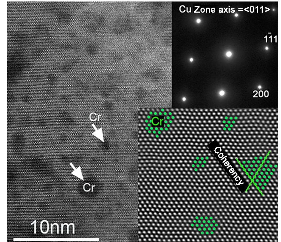
Figure: An atomic-resolution, high-angle annular dark-field image of an aged sample showing uniformly distributed Cr precipitates (dark contrast in main image). A fast Fourier transformed image (lower inset) shows coherent interfaces (such as the one indicated by a green line) between the Cu matrix and the precipitates (shown in green). Due to the coherent structure between the precipitates and the matrix, only one set of diffraction spots appears in the selected area diffraction pattern (top inset).
