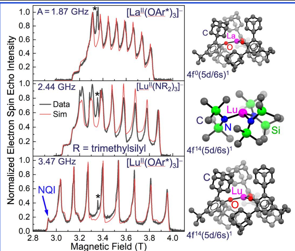
Figure. Pulsed electron spin-echo spectra recorded at 94GHz and 5K, for the three compounds shown. The eight ( = 2I + 1 ) lines arise due to the hyperfine interaction (HFI) with the I = 7/2 ^{175}\text{Lu} or ^{139}\text{La} nuclear spin; the spacing between peaks is a direct measure of the HFI strength, A , which increases from top to bottom. The asterisk marks an impurity and the “NQI” feature is attributed to a strong nuclear quadrupole interaction.
