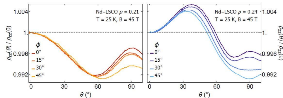
Angle-Dependent Magneto-Resistance (ADMR) data at a temperature of T=25\text{K} and at a magnetic field of B=45\text{T} from the cuprate superconductor Nd-LSCO as a function of magnetic field angle \theta . The data were taken (left) inside the pseudogap phase at carrier concentration p = 0.21 , and (right) outside the pseudogap phase at p=0.24 .
