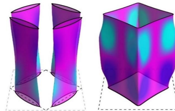
Fermi surfaces calculated from ADMR data (left) inside the pseudogap phase at p=0.21 , showing four small pockets (resembling those that would be created by antiferromagnetism) and (right) outside the pseudogap phase at p=0.24 , showing the single large pocket of a simple metal.
